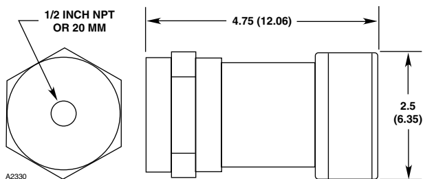
xWatch Dimensions in Inches (Centimeters)
