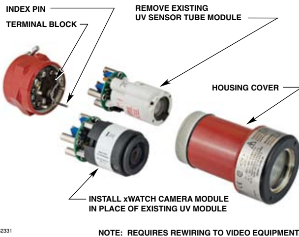
Converting C7050 to xWatch
